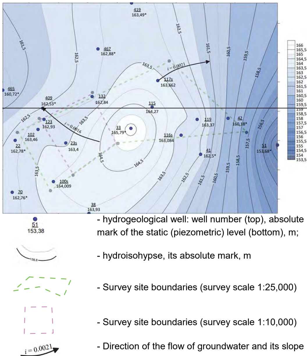
Figure 5.8 – Schematic map of the hydroisohypses of groundwater
