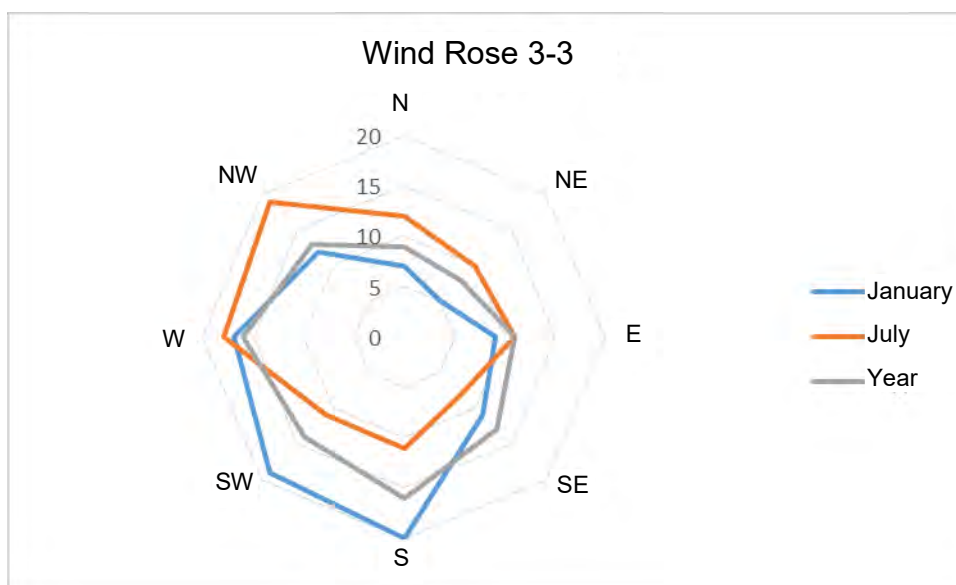
Figure 5.2. – Average annual wind rose
